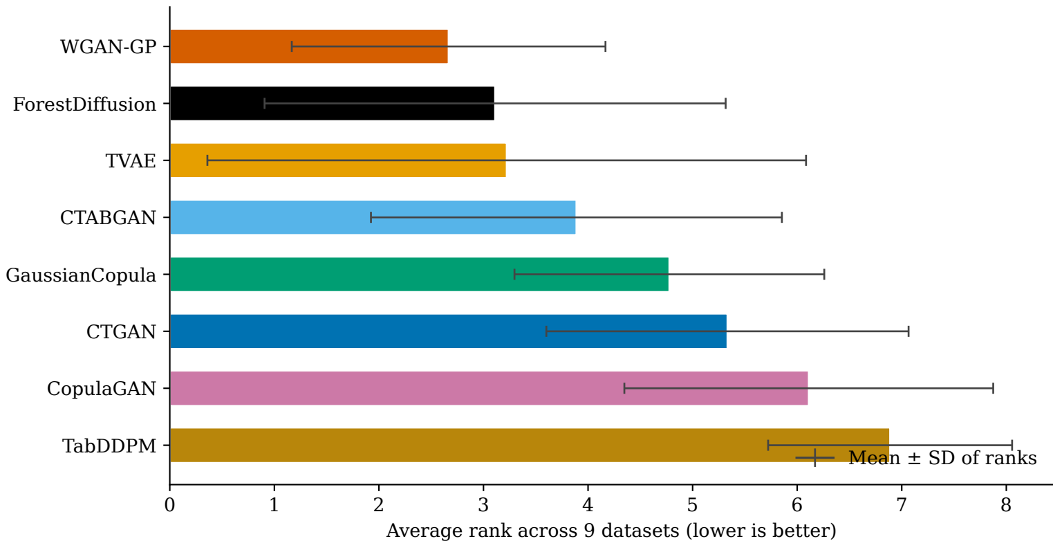
Generator Robustness — Average Accuracy-Gap Rank (10-seed means)
